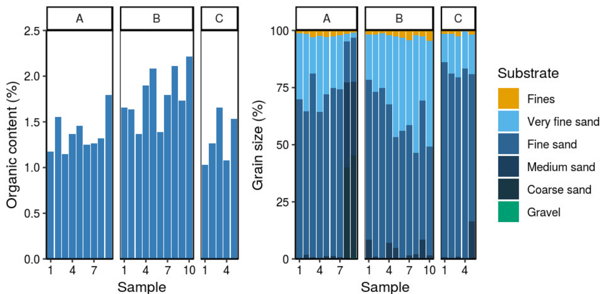
Figure 10: Sediment sample locations and characteristics at Eastern Beach. Labels correspond to stratum and sample number. Graphs show organic content (% dry weight) and cumulative grain size (%). Sediment grain size fractions include fines (silt and clay; <63 µm), sands (very fine, >63 µm; fine, >125 µm; medium, >250 µm; coarse, >500 µm), and gravel (>2000 µm) (see details in Table B-1).
