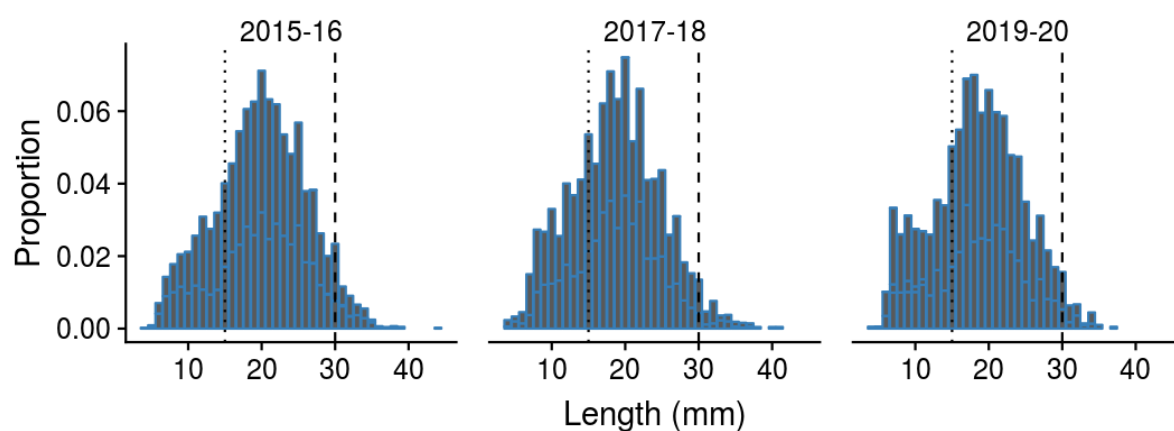
Figure 48: Weighted length-frequency (LF) distribution of cockles for the present and previous surveys at Whangateau Harbour. Vertical dotted and dashed lines indicate the cut-off sizes for recruits and large individuals, respectively.
