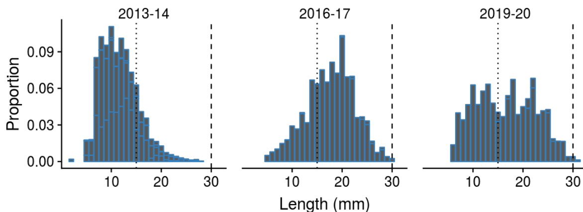
Figure 43: Weighted length-frequency (LF) distribution of cockles for the present and previous surveys at Waiōtahe Estuary. Vertical dotted and dashed lines indicate the cut-off sizes for recruits and large individuals, respectively.
