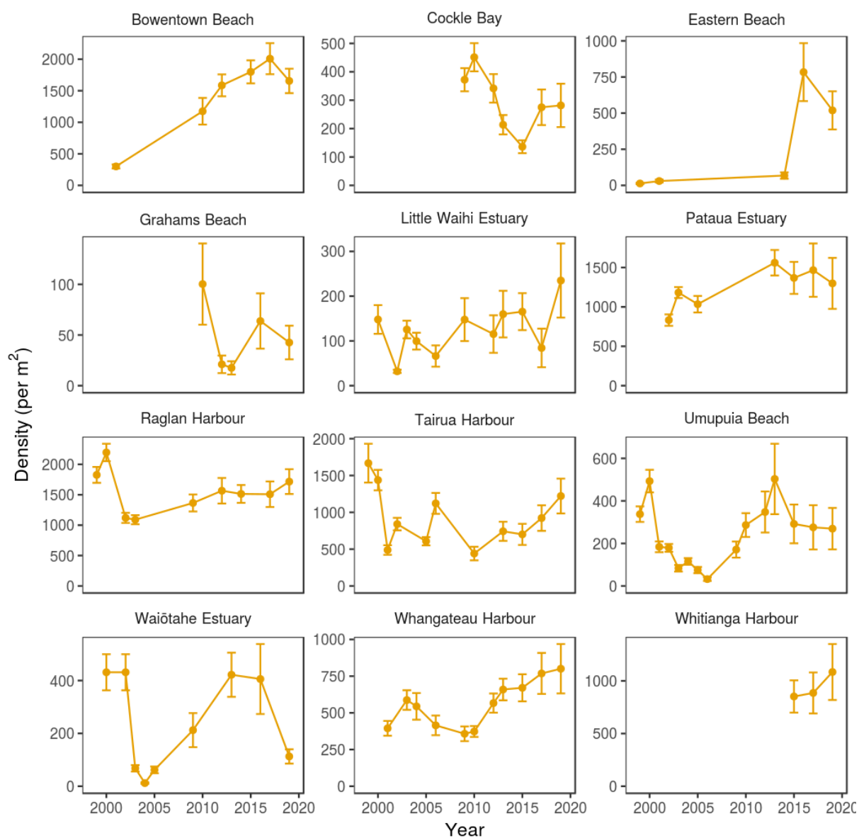
Figure 56: Estimated density of cockles for all sites included in the 2019–20 survey. Shown are the mean estimated densities across years, with bars indicating the 95% confidence interval. (Note different scales on the y-axes. Not all sites were surveyed each year, and the sampling extent may vary across years.)
