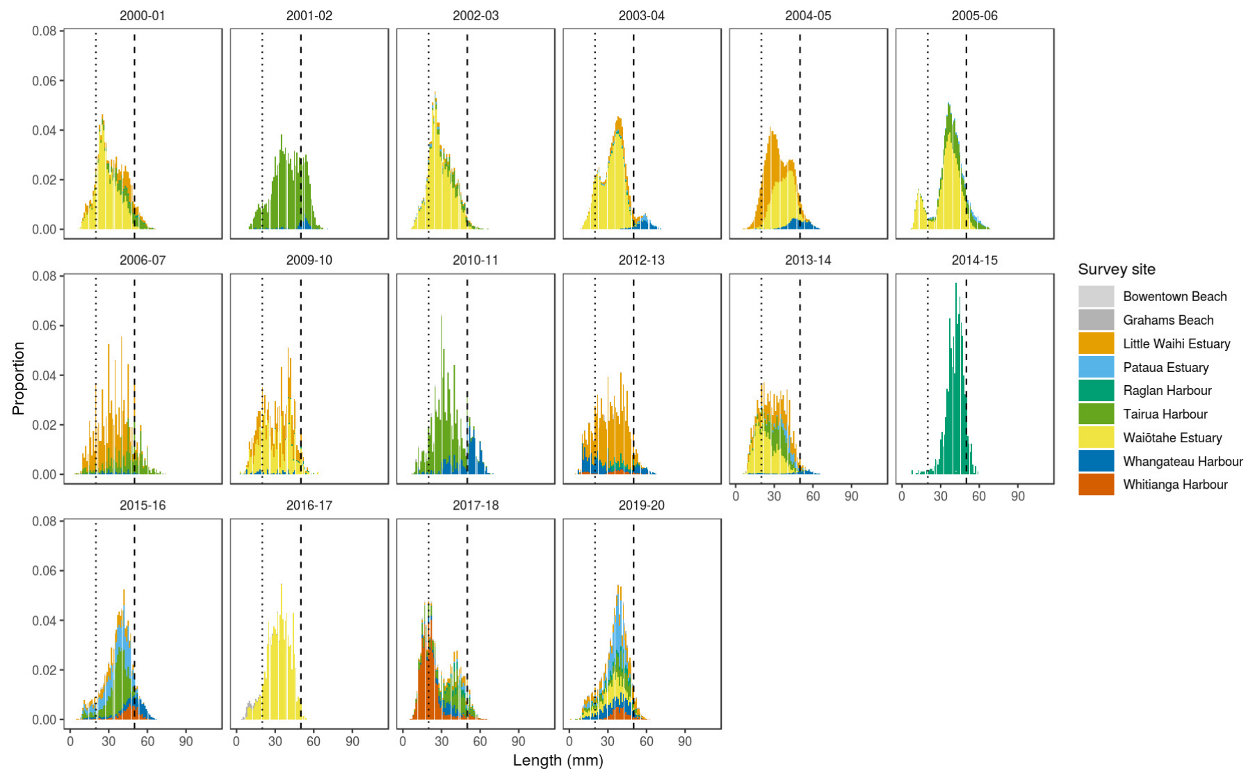
Figure 60: Weighted length-frequency (LF) distributions of pipi over time at sites included in the 2019–20 survey. LF distributions were estimated independently for all strata in each survey to provide the total LF distribution. Vertical dotted and dashed lines indicate the cut-off sizes for recruits and large individuals, respectively. (Note, not all sites were surveyed each year, and the sampling extent may vary across years.)
