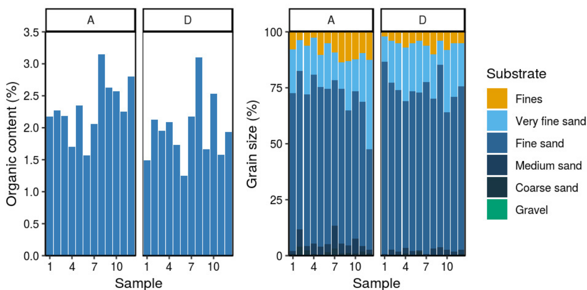
Figure 28: Sediment sample locations and characteristics at Raglan Harbour. Labels correspond to stratum and sample number. Graphs show organic content (% dry weight) and cumulative grain size (%). Sediment grain size fractions include fines (silt and clay; <63\ \mu\text{m} ), sands (very fine, >63\ \mu\text{m} ; fine, >125\ \mu\text{m} ; medium, >250\ \mu\text{m} ; coarse, >500\ \mu\text{m} ), and gravel ( >2000\ \mu\text{m} ) (see details in Table B-1).
