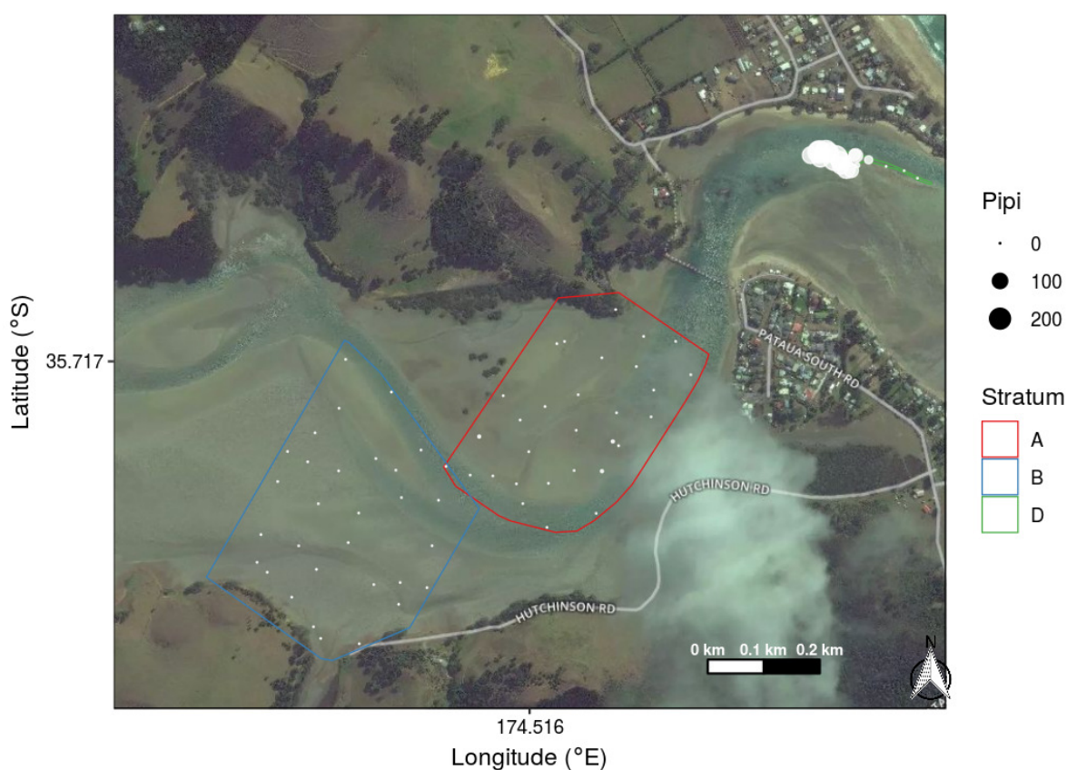
Figure 26: Map of sample strata and individual sample locations for pipi at Pataua Estuary, with the size of the circles proportional to the number of pipi (per 0.035 m 2 ) found at each location. Samples with zero counts are shown as small dots.
