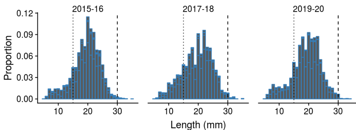
Figure 35: Weighted length-frequency (LF) distribution of cockles for the present and previous surveys at Tairua Harbour. Vertical dotted and dashed lines indicate the cut-off sizes for recruits and large individuals, respectively.
