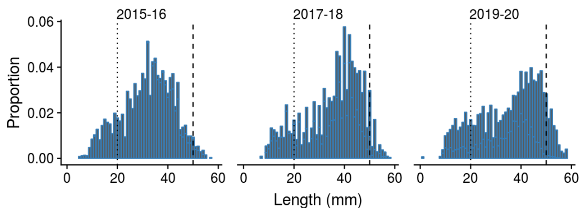
Figure 22: Weighted length-frequency (LF) distribution of pipi for the present and previous surveys at Little Waihi Estuary. Vertical dotted and dashed lines indicate the cut-off sizes for recruits and large individuals, respectively.
