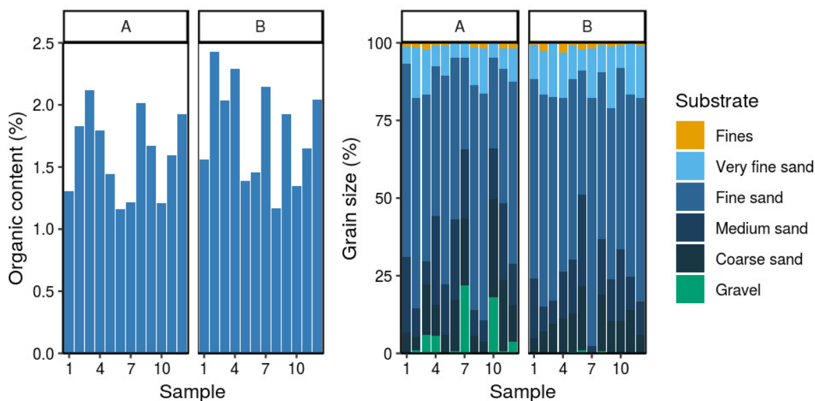
Figure 23: Sediment sample locations and characteristics at Pataua Estuary. Labels correspond to stratum and sample number. Graphs show organic content (% dry weight) and cumulative grain size (%). Sediment grain size fractions include fines (silt and clay; <63\ \mu\text{m} ), sands (very fine, >63\ \mu\text{m} ; fine, >125\ \mu\text{m} ; medium, >250\ \mu\text{m} ; coarse, >500\ \mu\text{m} ), and gravel ( >2000\ \mu\text{m} ) (see details in Table B-1).
