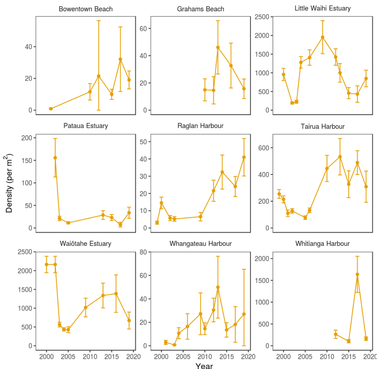
Figure 59: Estimated density of pipi for all sites included in the 2019–20 survey. Shown are the mean estimated densities across years, with bars indicating the 95% confidence interval. (Note different scales on the y-axes. Not all sites were surveyed each year, and the sampling extent may vary across years.)
