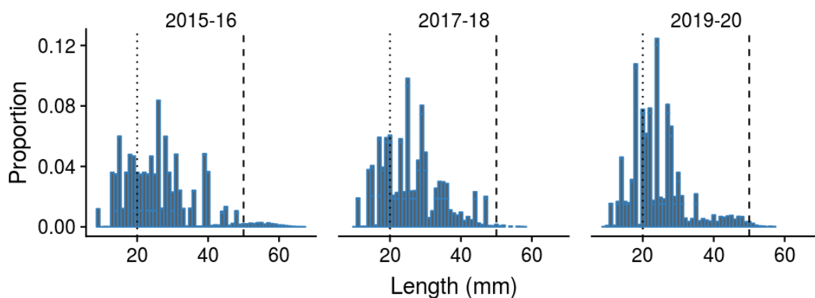
Figure 50: Weighted length-frequency (LF) distribution of pipi for the present and previous surveys at Whangateau Harbour. Vertical dotted and dashed lines indicate the cut-off sizes for recruits and large individuals, respectively.
