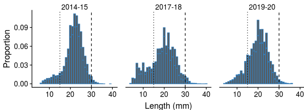
Figure 30: Weighted length-frequency (LF) distribution of cockles for the present and previous surveys at Raglan Harbour. Vertical dotted and dashed lines indicate the cut-off sizes for recruits and large individuals, respectively.
