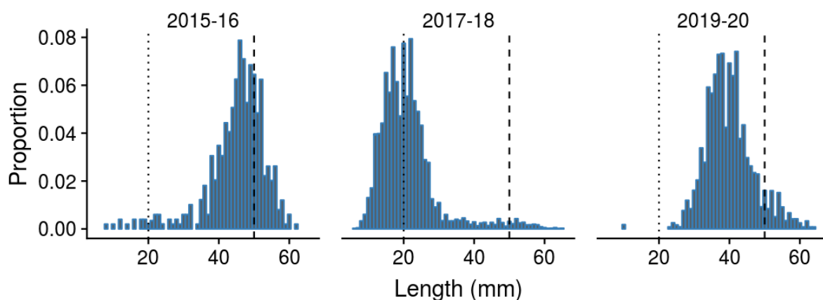
Figure 55: Weighted length-frequency (LF) distribution of pipi for the present and previous surveys at Whitianga Harbour. Vertical dotted and dashed lines indicate the cut-off sizes for recruits and large individuals, respectively.
