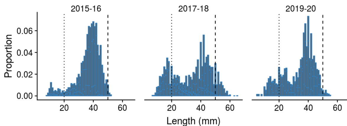
Figure 37: Weighted length-frequency (LF) distribution of pipi for the present and previous surveys at Tairua Harbour. Vertical dotted and dashed lines indicate the cut-off sizes for recruits and large individuals, respectively.
