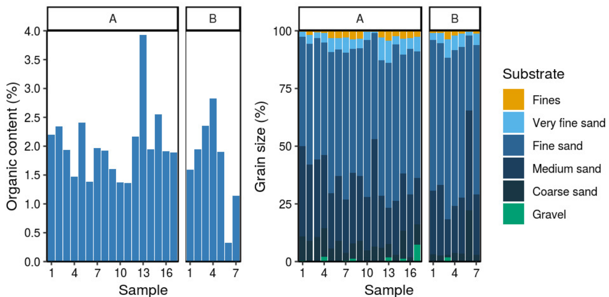
Figure 18: Sediment sample locations and characteristics at Little Waihi Estuary. Labels correspond to stratum and sample number. Graphs show organic content (% dry weight) and cumulative grain size (%). Sediment grain size fractions include fines (silt and clay; <63\ \mu\text{m} ), sands (very fine, >63\ \mu\text{m} ; fine, >125\ \mu\text{m} ; medium, >250\ \mu\text{m} ; coarse, >500\ \mu\text{m} ), and gravel ( >2000\ \mu\text{m} ) (see details in Table B-1).
