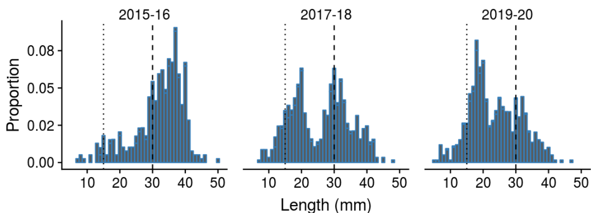
Figure 9: Weighted length-frequency (LF) distribution of cockles for the present and previous surveys at Cockle Bay. Vertical dotted and dashed lines indicate the cut-off sizes for recruits and large individuals, respectively.
