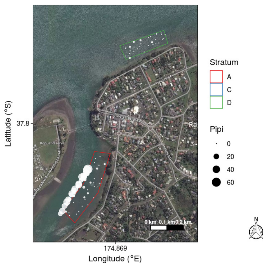
Figure 31: Map of sample strata and individual sample locations for pipi at Raglan Harbour, with the size of the circles proportional to the number of pipi (per 0.035 m 2 ) found at each location. Samples with zero counts are shown as small dots.
