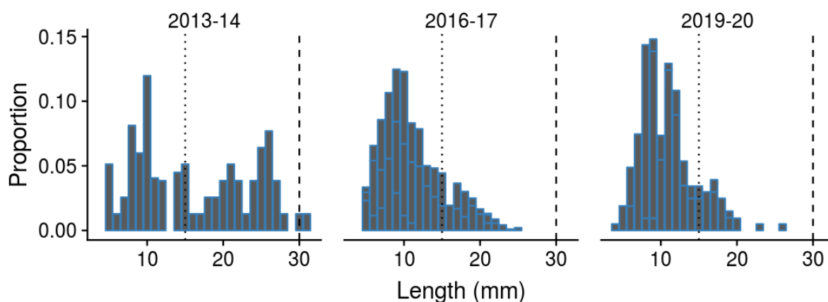
Figure 15: Weighted length-frequency (LF) distribution of cockles for the present and previous surveys at Grahams Beach. Vertical dotted and dashed lines indicate the cut-off sizes for recruits and large individuals, respectively.
