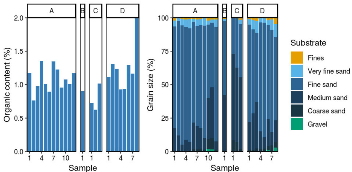
Figure 46: Sediment sample locations and characteristics at Whangateau Harbour. Labels correspond to stratum and sample number. Graphs show organic content (% dry weight) and cumulative grain size (%). Sediment grain size fractions include fines (silt and clay; <63 µm), sands (very fine, >63 µm; fine, >125 µm; medium, >250 µm; coarse, >500 µm), and gravel (>2000 µm) (see details in Table B-1).
