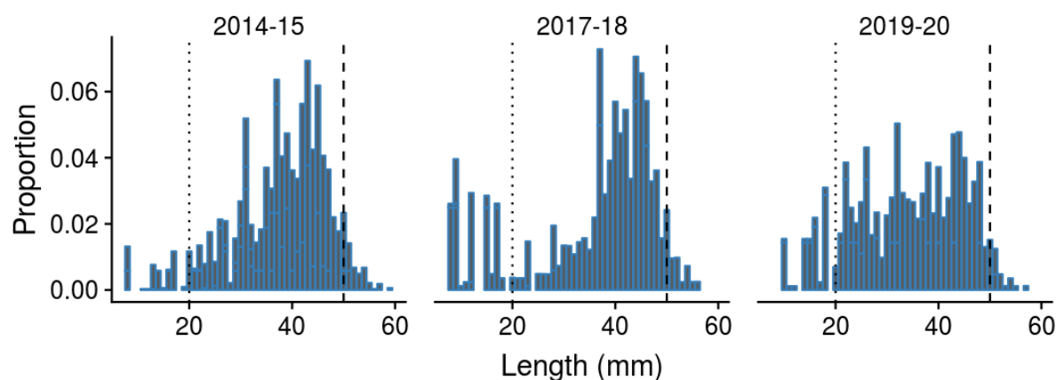
Figure 32: Weighted length-frequency (LF) distribution of pipi for the present and previous surveys at Raglan Harbour. Vertical dotted and dashed lines indicate the cut-off sizes for recruits and large individuals, respectively.
