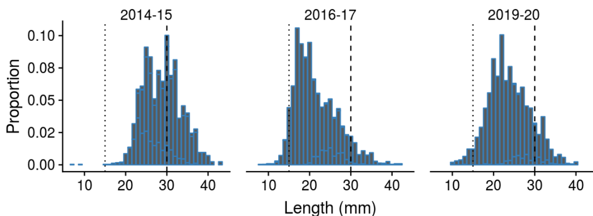
Figure 12: Weighted length-frequency (LF) distribution of cockles for the present and previous surveys at Eastern Beach. Vertical dotted and dashed lines indicate the cut-off sizes for recruits and large individuals, respectively.
