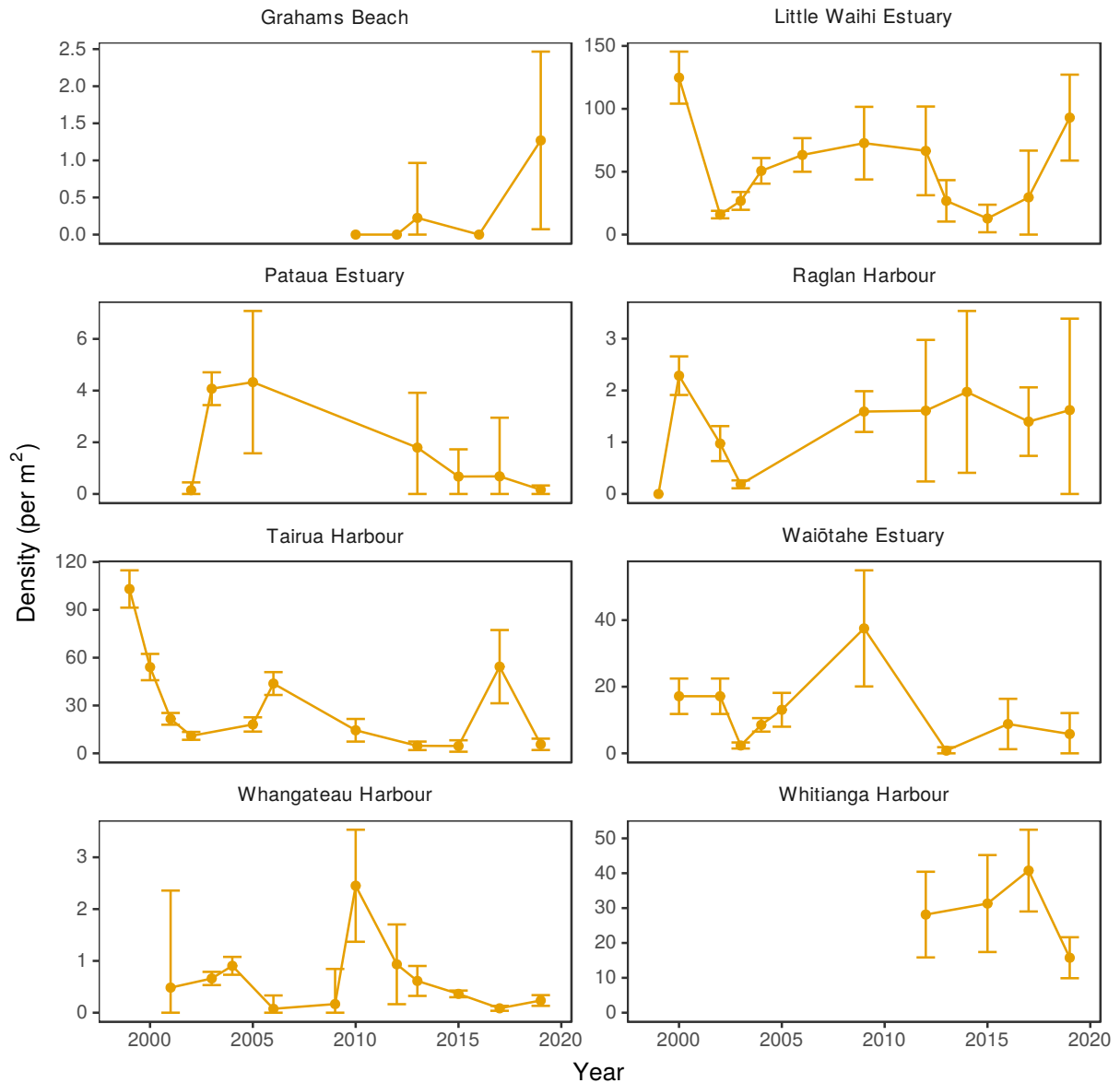
Figure 61: Estimated density of large pipi (≥50 mm shell length) for all sites where pipi in this size class were present in at least one survey. Shown are the mean estimated densities across years, with bars indicating the 95% confidence interval. (Note, different scales on the y-axes. Not all sites were surveyed each year, and the sampling extent may vary across years.)
