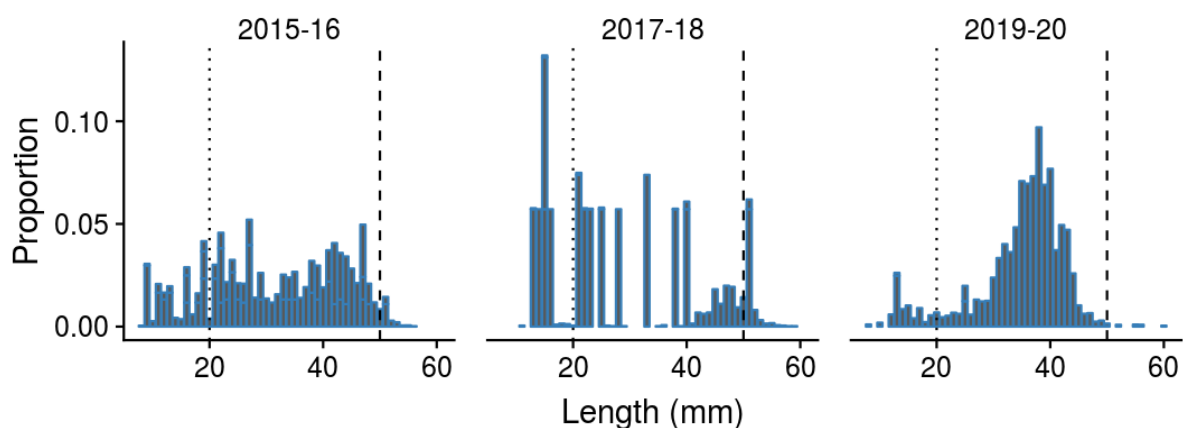
Figure 27: Weighted length-frequency (LF) distribution of pipi for the present and previous surveys at Pataua Estuary. Vertical dotted and dashed lines indicate the cut-off sizes for recruits and large individuals, respectively.
