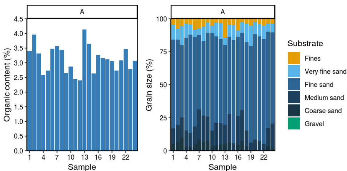
Figure 51: Sediment sample locations and characteristics at Whitianga Harbour. Labels correspond to stratum and sample number. Graphs show organic content (% dry weight) and cumulative grain size (%). Sediment grain size fractions include fines (silt and clay; <63\ \mu\text{m} ), sands (very fine, >63\ \mu\text{m} ; fine, >125\ \mu\text{m} ; medium, >250\ \mu\text{m} ; coarse, >500\ \mu\text{m} ), and gravel ( >2000\ \mu\text{m} ) (see details in Table B-1).
