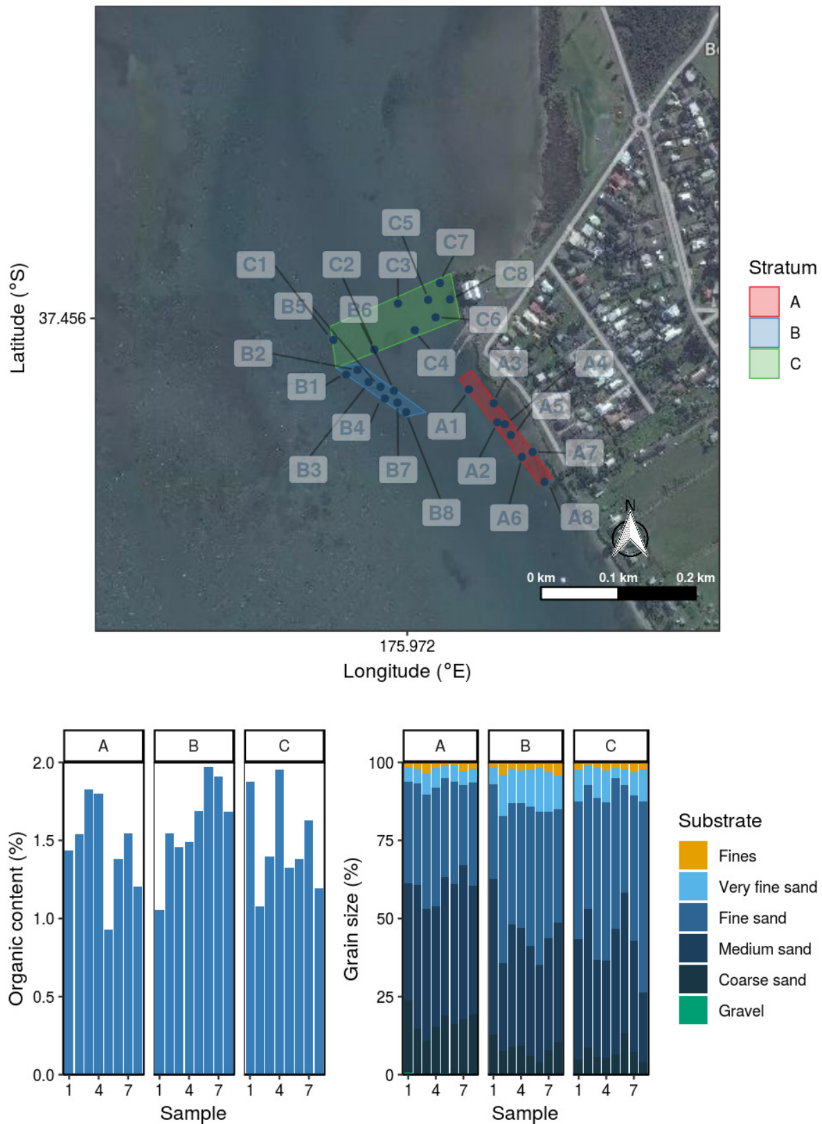
Figure 2: Sediment sample locations and characteristics at Bowentown Beach. Labels correspond to stratum and sample number. Graphs show organic content (% dry weight) and cumulative grain size (%). Sediment grain size fractions include fines (silt and clay; <63\ \mu\text{m} ), sands (very fine, >63\ \mu\text{m} ; fine, >125\ \mu\text{m} ; medium, >250\ \mu\text{m} ; coarse, >500\ \mu\text{m} ), and gravel ( >2000\ \mu\text{m} ) (see details in Table B-1).
