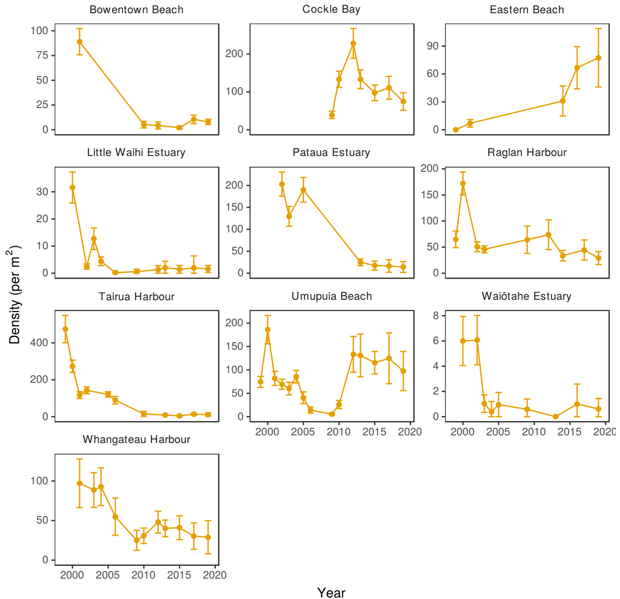
Figure 58: Estimated density of large cockles ( \geq 30 mm shell length) for all sites where cockles in this size class were present in at least one survey. Shown are the mean estimated densities across years, with bars indicating the 95% confidence interval. (Note, different scales on the y-axes. Not all sites were surveyed each year, and the sampling extent may vary across years.)
