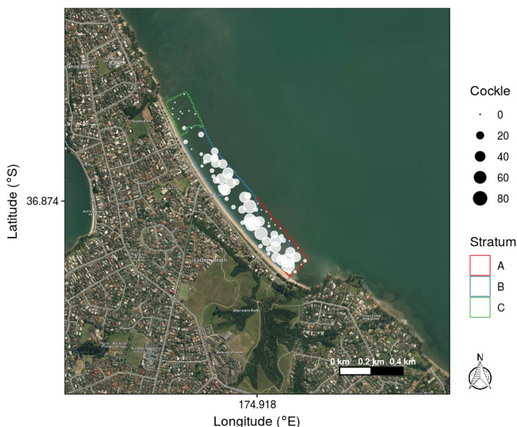
Figure 11: Map of sample strata and individual sample locations for cockles at Eastern Beach, with the size of the circles proportional to the number of cockles (per 0.035 m 2 ) found at each location. Samples with zero counts are shown as small dots.
