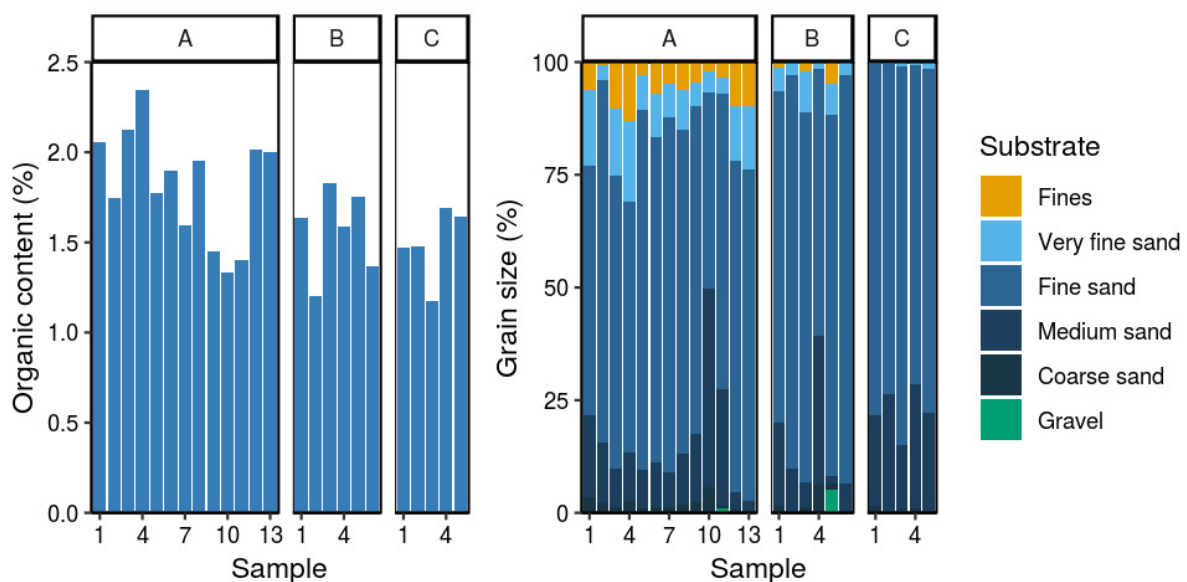
Figure 41: Sediment sample locations and characteristics at Waiōtahe Estuary. Labels correspond to stratum and sample number. Graphs show organic content (% dry weight) and cumulative grain size (%). Sediment grain size fractions include fines (silt and clay; <63 \mu\text{m} ), sands (very fine, >63 \mu\text{m} ; fine, >125 \mu\text{m} ; medium, >250 \mu\text{m} ; coarse, >500 \mu\text{m} ), and gravel (>2000 \mu\text{m} ) (see details in Table B-1).
