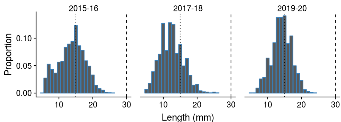
Figure 53: Weighted length-frequency (LF) distribution of cockles for the present survey at Whitianga Harbour. Vertical dotted and dashed lines indicate the cut-off sizes for recruits and large individuals, respectively.
