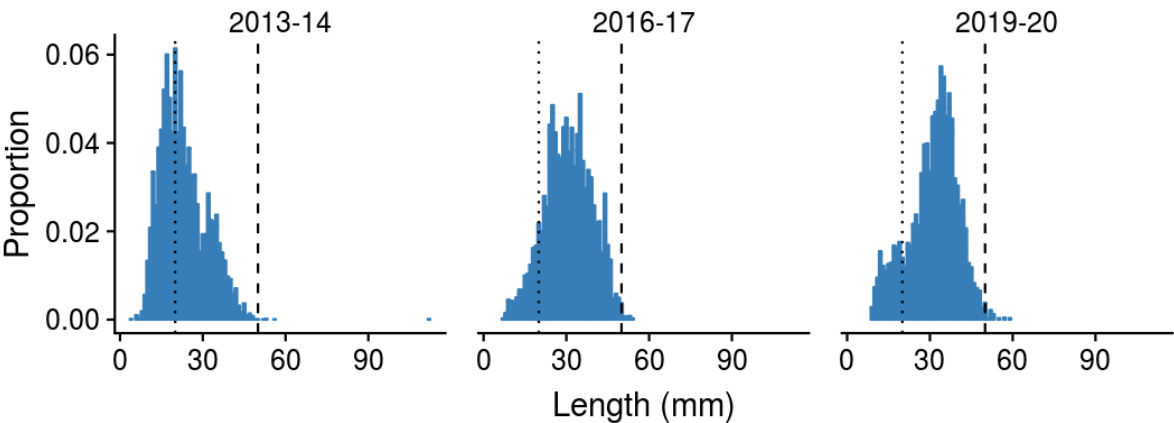
Figure 45: Weighted length-frequency (LF) distribution of pipi for the present and previous surveys at Waiōtahe Estuary. Vertical dotted and dashed lines indicate the cut-off sizes for recruits and large individuals, respectively.
