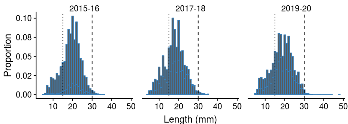
Figure 25: Weighted length-frequency (LF) distribution of cockles for the present and previous surveys at Pataua Estuary. Vertical dotted and dashed lines indicate the cut-off sizes for recruits and large individuals, respectively.
