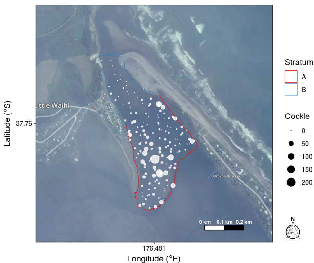
Figure 19: Map of sample strata and individual sample locations for cockles at Little Waihi Estuary, with the size of the circles proportional to the number of cockles (per 0.035 m 2 ) found at each location. Samples with zero counts are shown as small dots.
