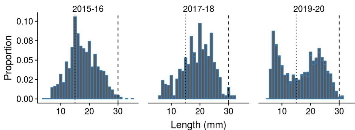
Figure 20: Weighted length-frequency (LF) distribution of cockles for the present and previous surveys at Little Waihi Estuary. Vertical dotted and dashed lines indicate the cut-off sizes for recruits and large individuals, respectively.
