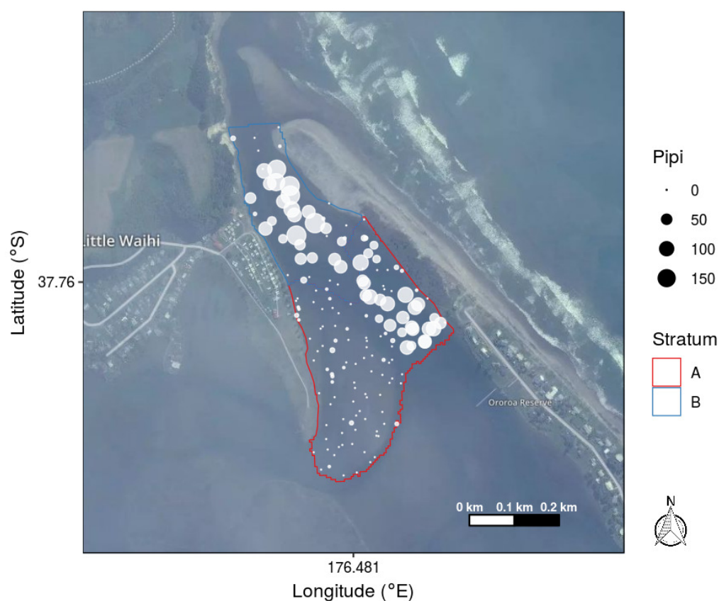
Figure 21: Map of sample strata and individual sample locations for pipi at Little Waihi Estuary, with the size of the circles proportional to the number of pipi (per 0.035 m 2 ) found at each location. Samples with zero counts are shown as small dots.
