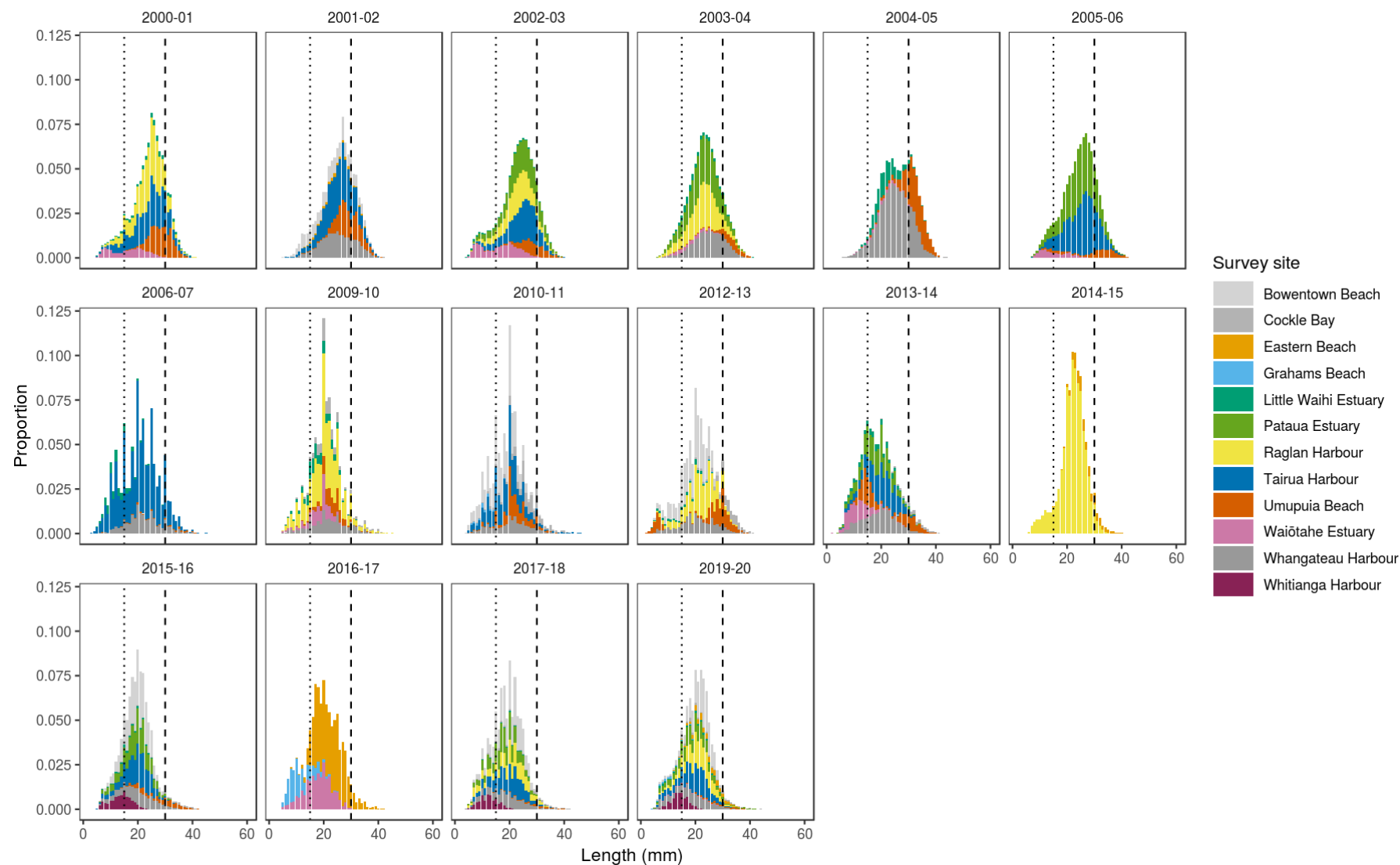
Figure 57: Weighted length-frequency (LF) distributions of cockles over time at sites included in the 2019–20 survey. LF distributions were estimated independently for all strata in each survey to provide the total LF distribution. Vertical dotted and dashed lines indicate the cut-off sizes for recruits and large individuals, respectively. (Note, not all sites were surveyed each year, and the sampling extent may vary across years.)
