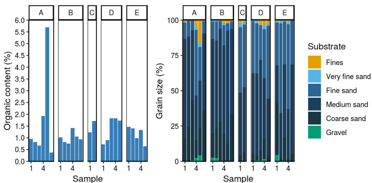
Figure 13: Sediment sample locations and characteristics at Grahams Beach. Labels correspond to stratum and sample number. Graphs show organic content (% dry weight) and cumulative grain size (%). Sediment grain size fractions include fines (silt and clay; <63 \mu\text{m} ), sands (very fine, >63 \mu\text{m} ; fine, >125 \mu\text{m} ; medium, >250 \mu\text{m} ; coarse, >500 \mu\text{m} ), and gravel ( >2000 \mu\text{m} ) (see details in Table B-1).
