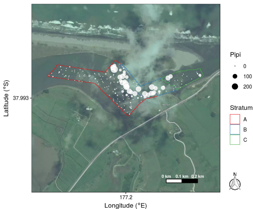
Figure 44: Map of sample strata and individual sample locations for pipi at Waiōtahe Estuary, with the size of the circles proportional to the number of pipi (per 0.035 m 2 ) found at each location. Samples with zero counts are shown as small dots.
