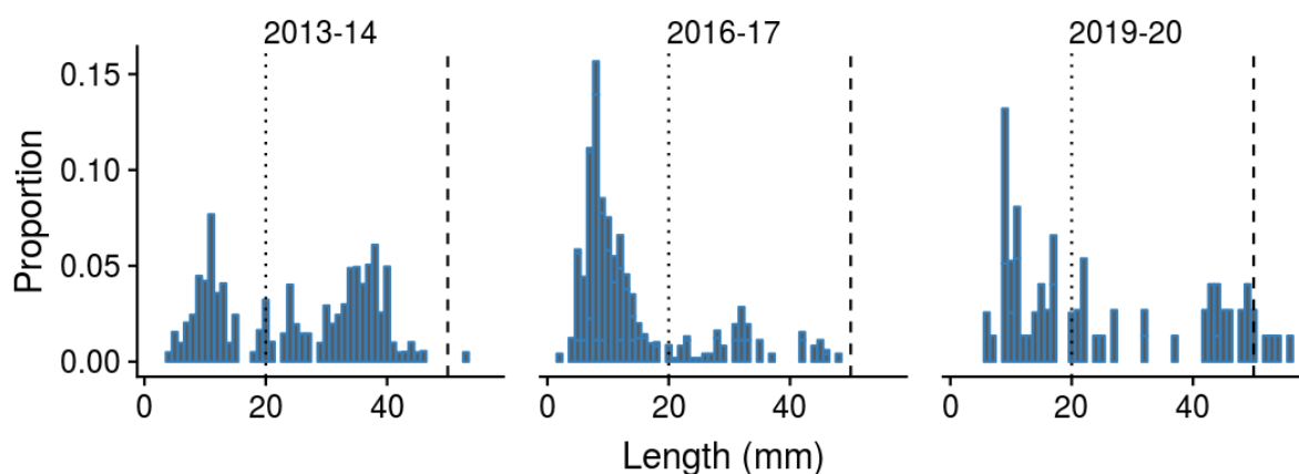
Figure 17: Weighted length-frequency (LF) distribution of pipi for the present and previous surveys at Grahams Beach. Vertical dotted and dashed lines indicate the cut-off sizes for recruits and large individuals, respectively.
