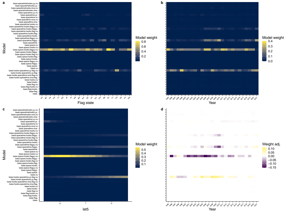
Figure 16: Model weight (geometric mean by stratum) for longline models by (a) vessel flag state, (b) year, and (c) latitude. The stacking-model weight adjustments between the training and prediction datasets by year are shown in (d).
