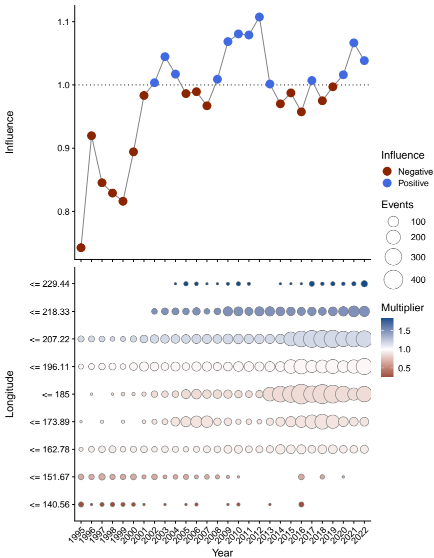
Figure B-28: Influence of longitude on catch-rates for sets, with positive influence showing years where the over - all catch - rate in the model was standardised downward by the corresponding amount to account for influences of longitude. Influence is shown in colour as a multiplier on average catch rates, with circle size corresponding to the amount of effort entering the model. Note that data for the 2022 year is preliminary.
